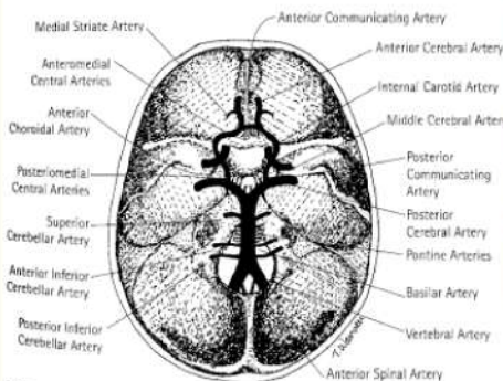
Fig. 4-1. Arteries/Circle of Willis
